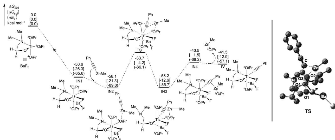
Figure 2. The DFT computed energy surfaces considered for zinc-to-titanium transmetalation. The values listed for each structure represent \Delta G_{298} , \Delta G_{\text{sol}} , and \Delta E_0 , respectively, in \text{kcal mol}^{-1} . Calculated bond lengths [Å]: Ti–N 2.532, Ti–O(1) 1.992, Ti–O(2) 2.146, Ti–O(3) 1.940, Ti–F 1.920, Ti–C 2.785, Ba–O(1) 2.744, Ba–F 2.553, Zn–O(3) 2.270, Zn–O(2) 2.076.
