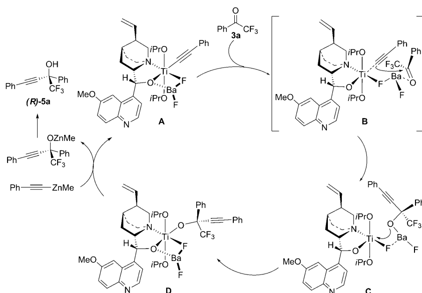
Scheme 1. Proposed mechanism and transition-state models for the alkynylation of 3a into 5a .
